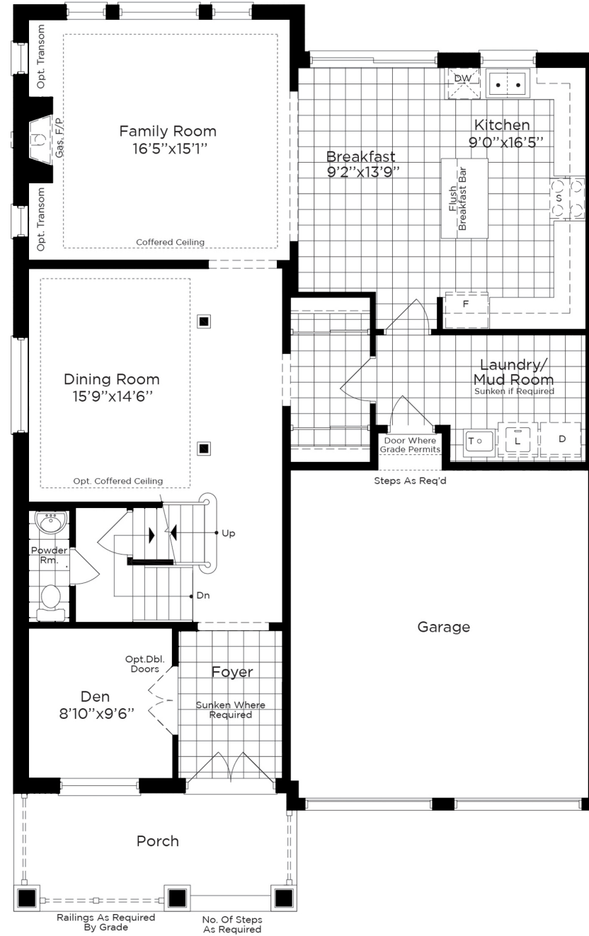
First Floor
